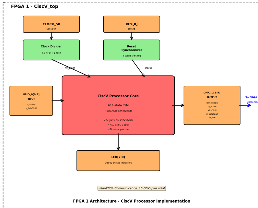
Figure 3: Complete system architecture of FPGA 1 hosting the CISC-V processor
