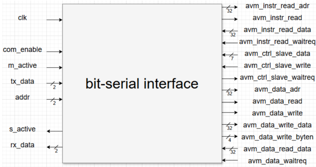
Figure 4: bit-serial interface architecture v1
