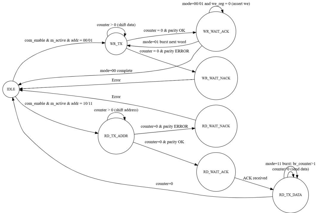
Figure 6: serialisation FSM graph
