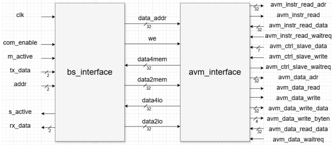
Figure 5: bit-serial interface architecture v2
